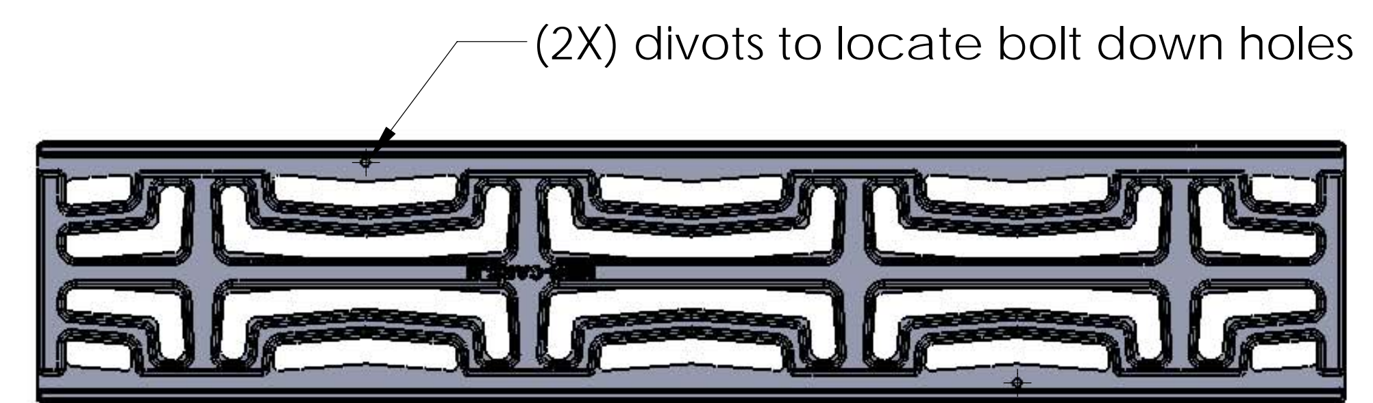
BOTTOM VIEW scale 1:3
